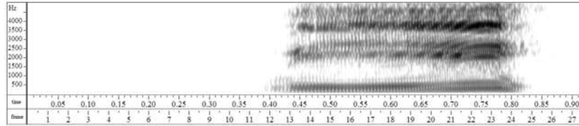
Figure 12: Sequence of stages in the articulation of /ʔbi s / ‘dipper’.
