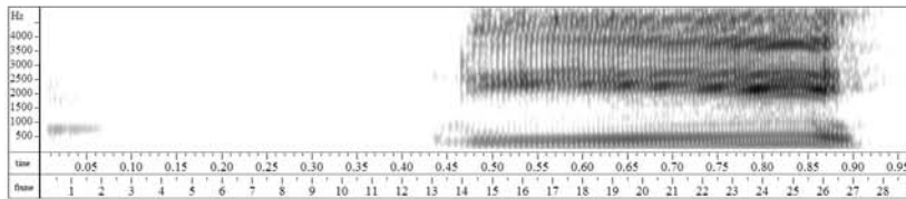
Figure 13: Sequence of stages in the articulation of /ʔdi s / ‘borrow money’.
