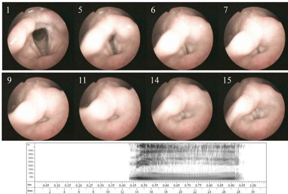
Figure 10: Sequence of stages in the articulation of /ʔmi¹/ ‘bear’ including laryngoscopic images and a spectrogram. Photographic frame numbers are indicated at the bottom of the spectrograms.
